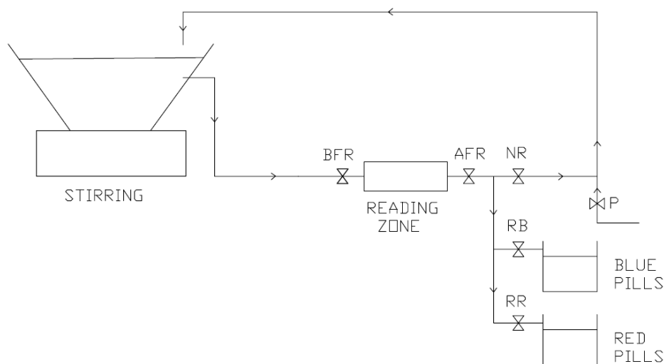
Figure 2. Scheme of pill analyser.
