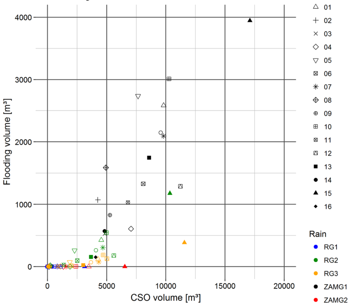
Figure 1. Flooding volume and CSO volume for measured 1 year rain series (RG 1 -3 and ZAMG 1 and 2) and the different calibration scenarios.
