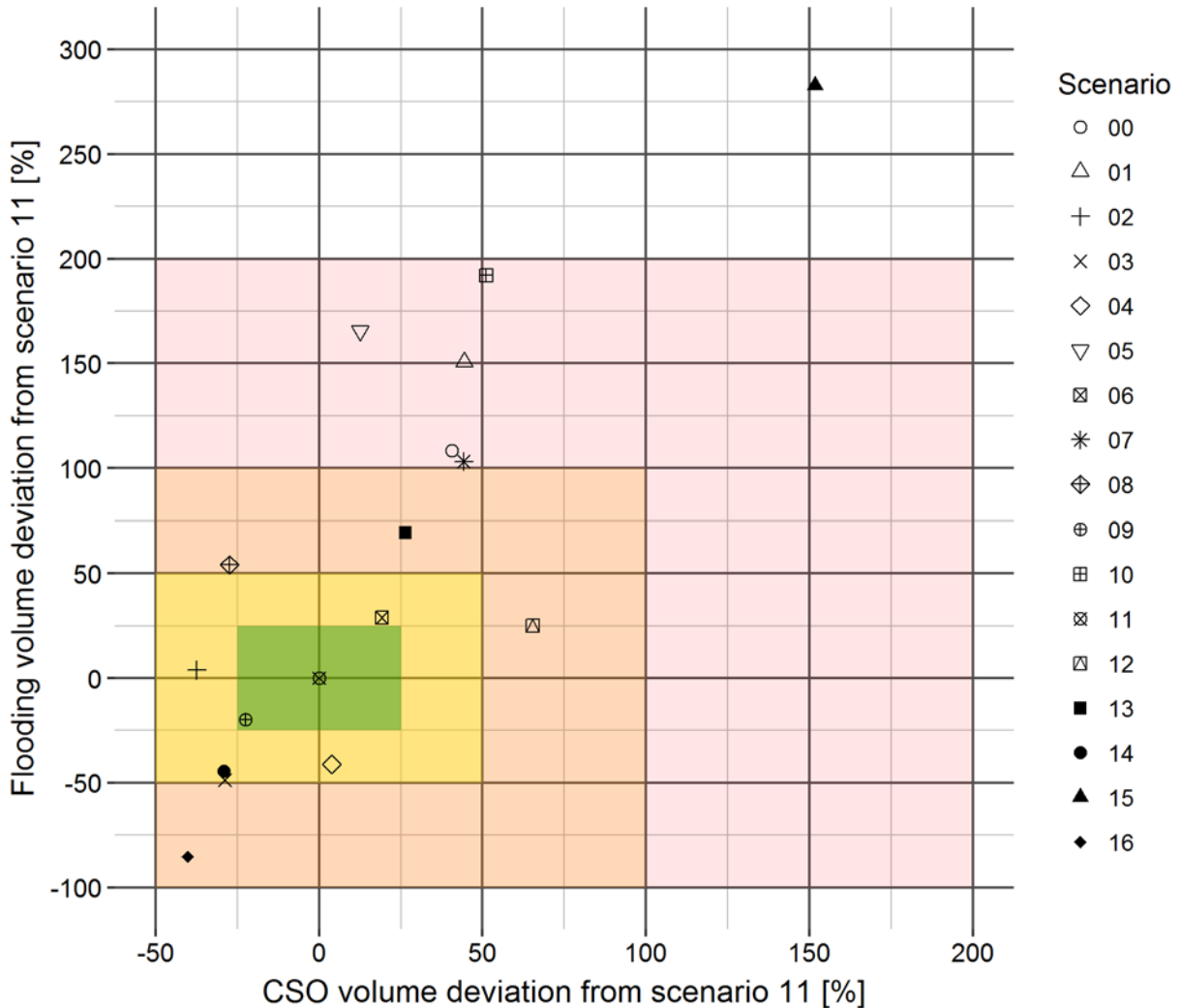
Figure 2. Flooding volume and CSO volume deviation from scenario 11 for measured 1 year rain series ZAMG 1
