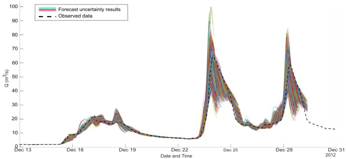
Figure 6 All forecast uncertainty results
