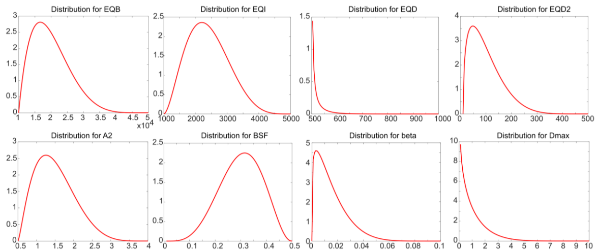
Figure 5 Probability distribution curve of the eight considered parameters at one sub-catchment
