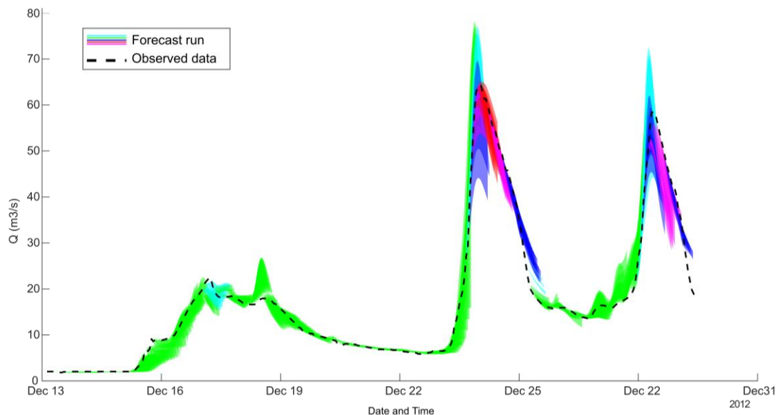
Figure 9 Observed discharge with updated forecasts
