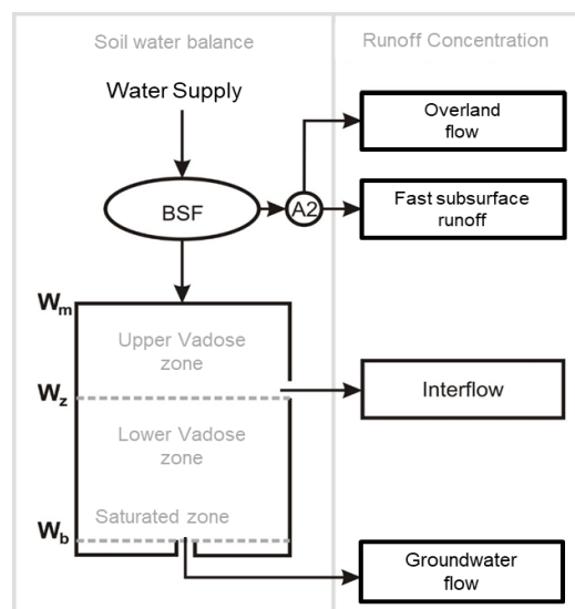
Figure 2 LARSIM water balance model
