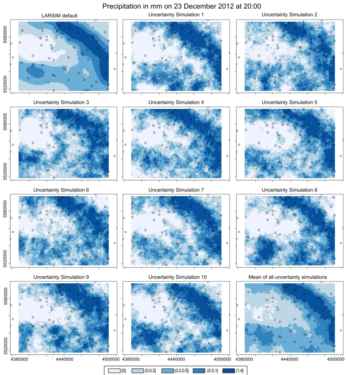
Figure 4 Uncertainty quantification of rainfall distribution
