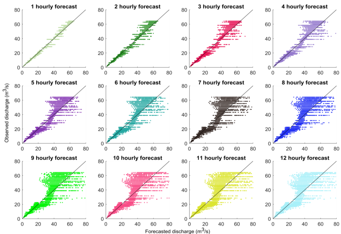
Figure 7 Scatter plots of observed vs simulated data for each hourly forecast leads
