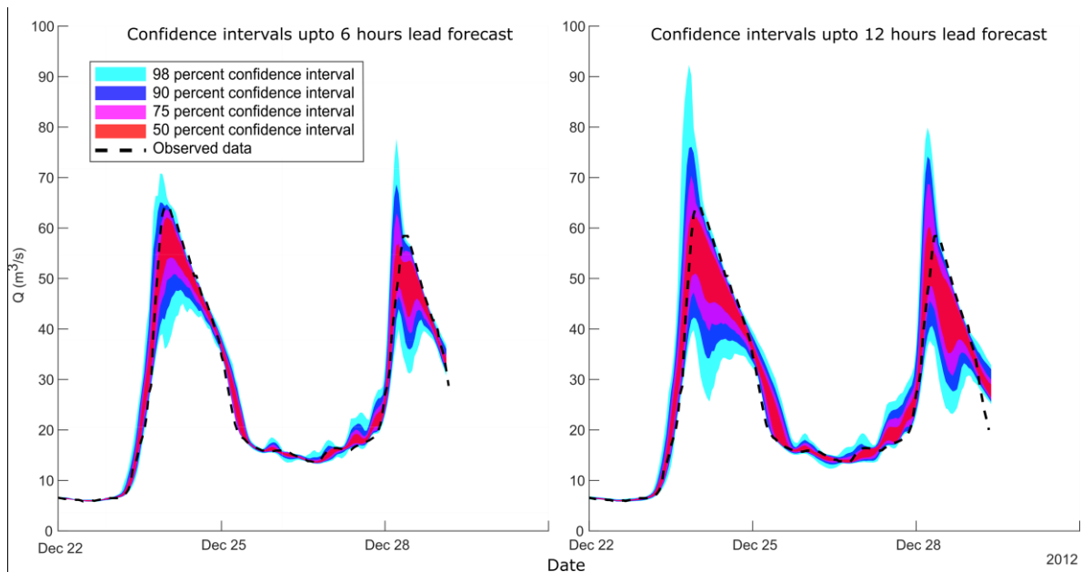
Figure 8 Confidence intervals in flood forecasting
