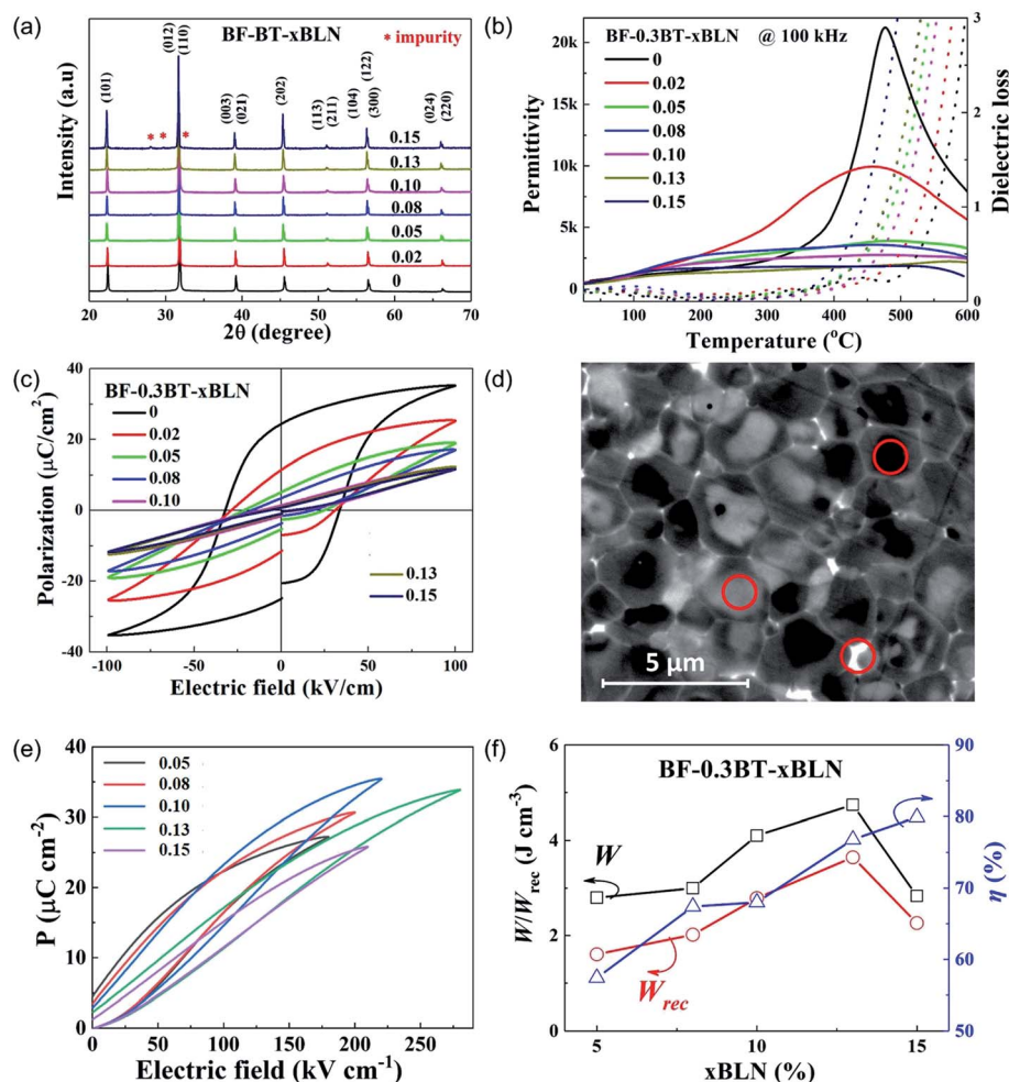
Fig. 2 (a) XRD patterns for BF–BT–xBLN ( x = 0.00 – 0.15 ). (b) Temperature-dependent permittivity and dielectric loss data for BF–BT–xBLN ceramics at a frequency of 100 kHz. (c) Bipolar P–E loops for BF–BT–xBLN ceramics (d) EDS elemental spot analysis (circled) for BF–BT–0.13BLN ceramics. (e) Unipolar P–E loops under E_{\max} and (f) energy storage properties under E_{\max} for BF–BT–xBLN ceramics.
