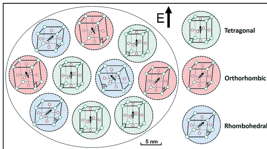
Fig. 10 A schematic illustration explaining the formation of a high strain E -induced pseudosymmetric state. Local distorted regions are shown as, but are not limited to, rhombohedral, tetragonal and orthorhombic symmetries.
