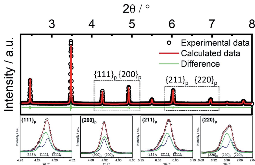
Fig. 1 High energy synchrotron XRD pattern and corresponding Rietveld refinement results for the unpoled BF-0.3BT ceramic with contributions of rhombohedral ( R3c ) and cubic ( Pm3m ) phases to individual peak profiles in the calculated pattern.
