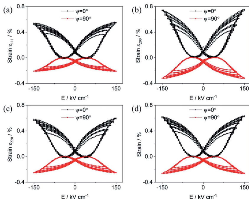
Fig. 9 Effective lattice strains calculated from single peak profiles of (a) \{111\}_p (b) \{200\}_p , (c) \{220\}_p peaks and (d) the E -induced lattice strain of BF-0.3BT-0.01NLN up to 150 \text{ kV cm}^{-1} at \beta = 0 and 90^\circ .
