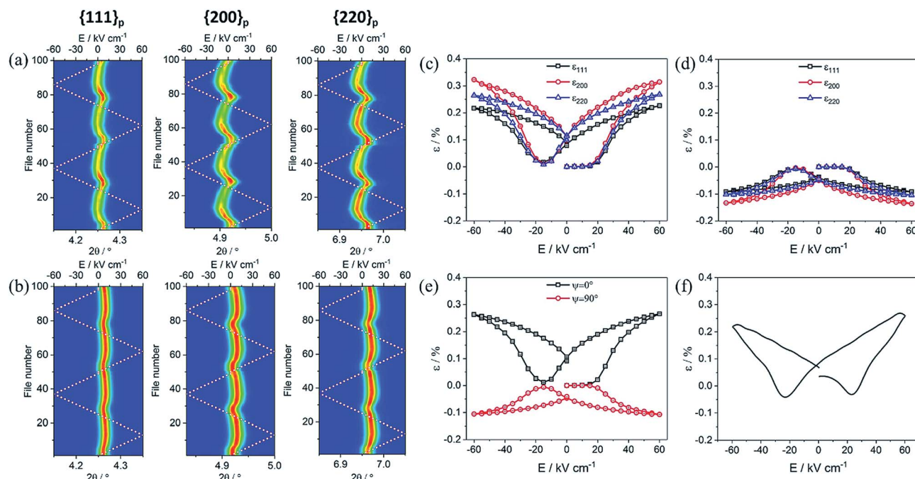
Fig. 5 Contour plots of the \{111\}_p , \{200\}_p and \{220\}_p peak profiles at (a) \beta = 0^\circ and (b) \beta = 90^\circ obtained from the in situ XRD experiment for BF-0.3BT-0.01NLN, with two cycles of electric field poling under \pm 60 \text{ kV cm}^{-1} ; effective lattice strains calculated from representative peaks with grain orientations of (c) \beta = 0^\circ and (d) \beta = 90^\circ for BF-0.3BT-0.01NLN; (e) the E -induced lattice strain for \beta = 0^\circ and \beta = 90^\circ for BF-0.3BT; (f) directly measured macroscopic S-E loop for BF-0.3BT-0.01NLN.
