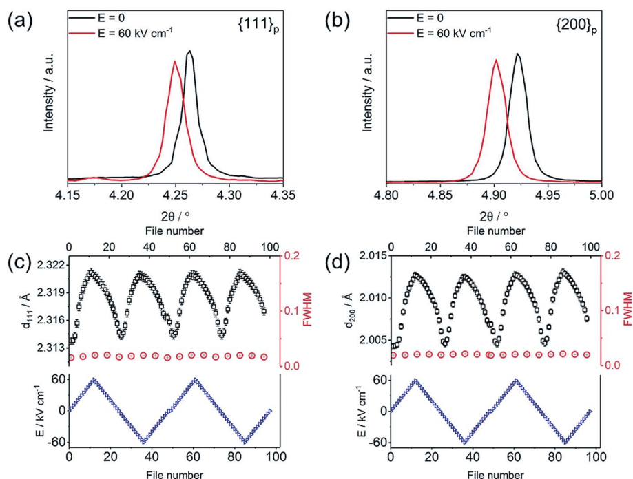
Fig. 6 (a) \{111\}_p and (b) \{200\}_p XRD peak profiles under 0 and 60 \text{ kV cm}^{-1} ; d -spacing and FWHM of (c) \{111\}_p and (d) \{200\}_p XRD peak profiles at \beta = 0^\circ obtained from the in situ XRD experiment for BF-0.3BT-0.01NLN, with two cycles of electric field poling under \pm 60 \text{ kV cm}^{-1} .
