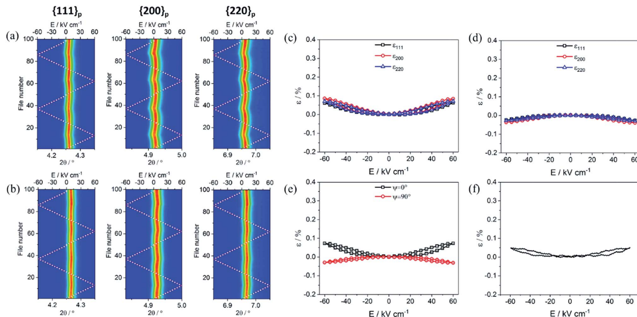
Fig. 7 Contour plots of the \{111\}_p , \{200\}_p and \{220\}_p peak profiles for (a) \beta = 0^\circ and (b) \beta = 90^\circ obtained from the in situ XRD experiment for BF-0.3BT-0.03NLN, with two cycles of electric field poling under \pm 60 \text{ kV cm}^{-1} ; effective lattice strains calculated from representative peaks with grain orientations of (c) \beta = 0^\circ and (d) \beta = 90^\circ for BF-0.3BT-0.03NLN; (e) the E -induced lattice strain for \beta = 0^\circ and \beta = 90^\circ for BF-0.3BT-0.03NLN; (f) directly measured macroscopic S-E loop for BF-0.3BT-0.03NLN.
