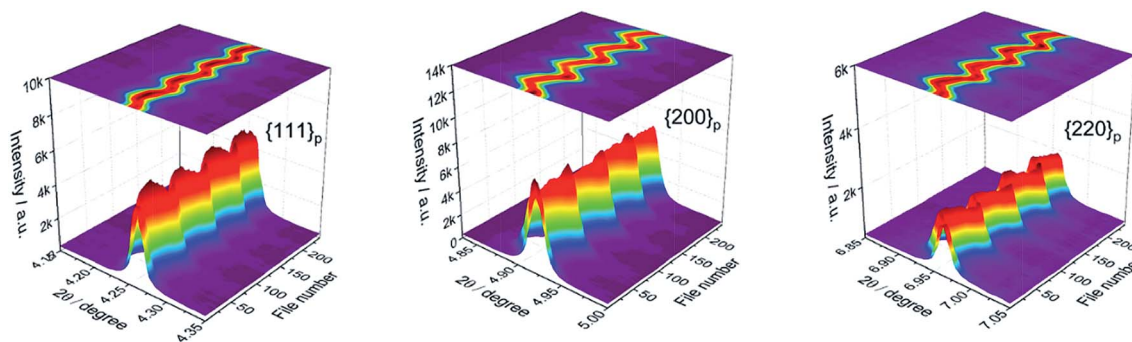
Fig. 8 Surface contour plots to illustrate changes in the \{111\}_p , \{200\}_p and \{220\}_p XRD peak profiles (at \beta = 0^\circ ) for BF-BT-0.01NLN under application of 2 cycles of electric field of \pm 150 \text{ kV cm}^{-1} .
