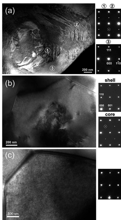
Fig. 3 TEM domain morphology with diffraction spots for (a) BF-0.3BT, (b) BF-0.3BT-0.01NLN and (c) BF-0.3BT-0.03NLN ceramics.
