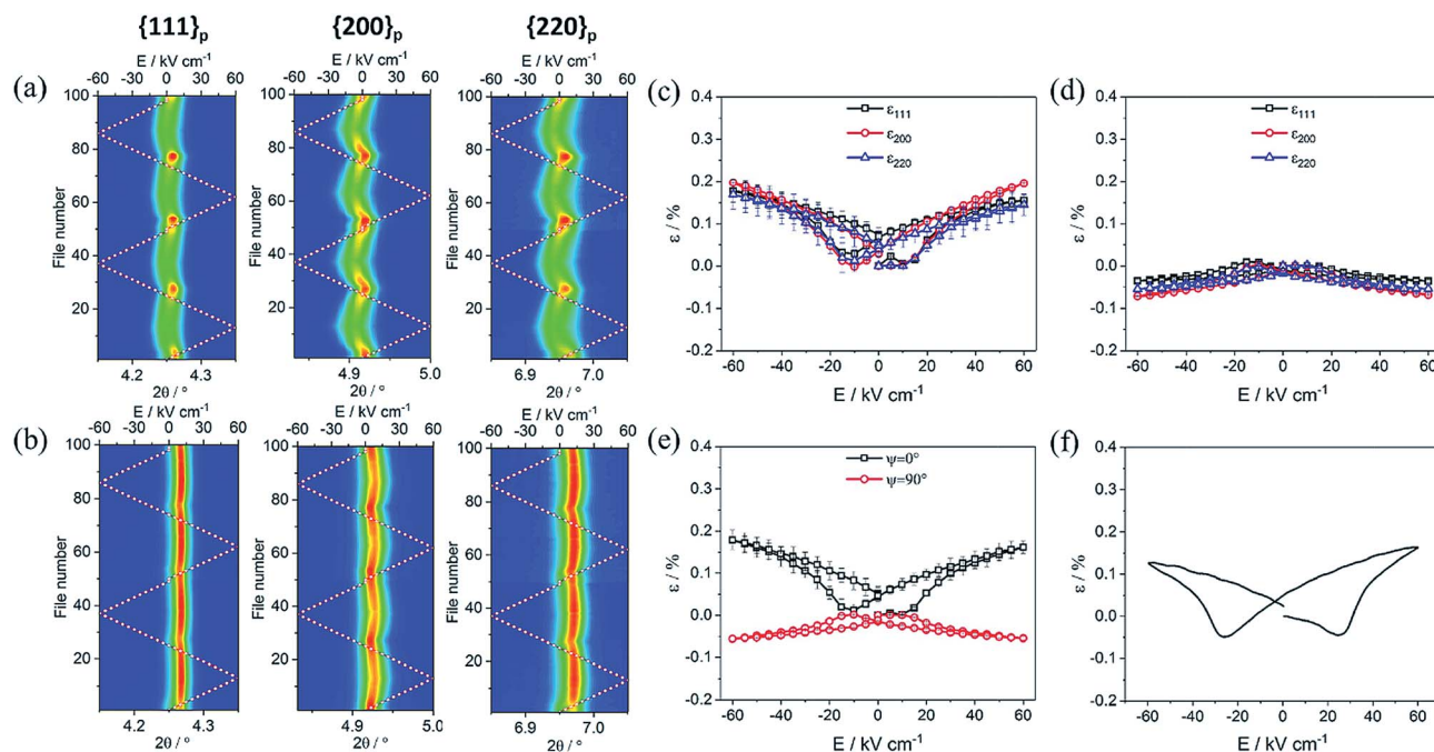
Fig. 4 Contour plots of the \{111\}_p , \{200\}_p and \{220\}_p peak profiles at (a) \beta = 0^\circ and (b) \beta = 90^\circ obtained from the in situ XRD experiment for BF-0.3BT, with two cycles of electric field poling under \pm 60 \text{ kV cm}^{-1} ; effective lattice strains calculated from representative peaks with grain orientation for (c) \beta = 0^\circ and (d) \beta = 90^\circ for BF-0.3BT; (e) the E -induced lattice strains for \beta = 0^\circ and \beta = 90^\circ for BF-0.3BT; (f) directly measured macroscopic S–E loop for BF-0.3BT.
