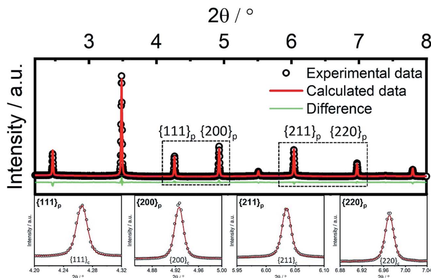
Fig. 2 High energy synchrotron XRD pattern and corresponding Rietveld refinement results for the unpoled BF-0.3BT-0.03NLN ceramic with a single cubic ( Pm3m ) phase indexed to individual peak profiles in the calculated pattern.
