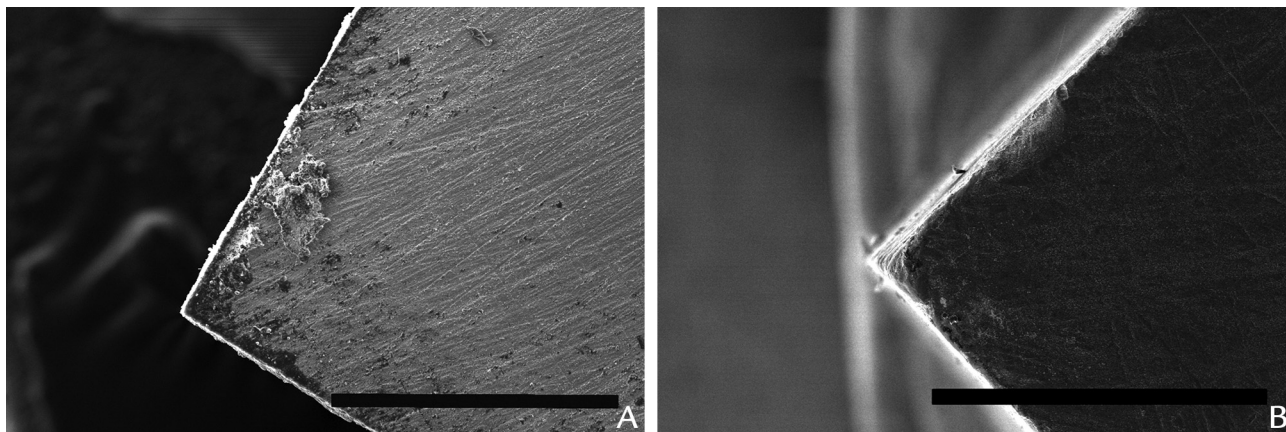
Figure 6. Scanning electron micrographs of Y-TZP. A, Before solubility testing (surface, edge, and corner). B, After solubility testing (surface, edge, and corner). Scale bar equals 500 \mu\text{m} . Original magnification \times 250 .
