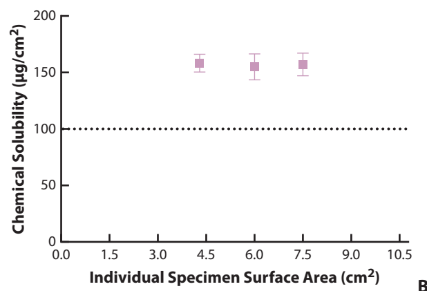
Figure 8. Comparison between average chemical solubility and individual surface area cubes (black) and spheres (gray). Dotted line demonstrates maximum acceptable chemical solubility (100 \mu\text{g}/\text{cm}^2 ) for enamel ceramics according to ISO 6872:2015 (bars represent standard deviation) ( n=3 ). A, Y-TZP. B, VITABLOCS Mark II.
