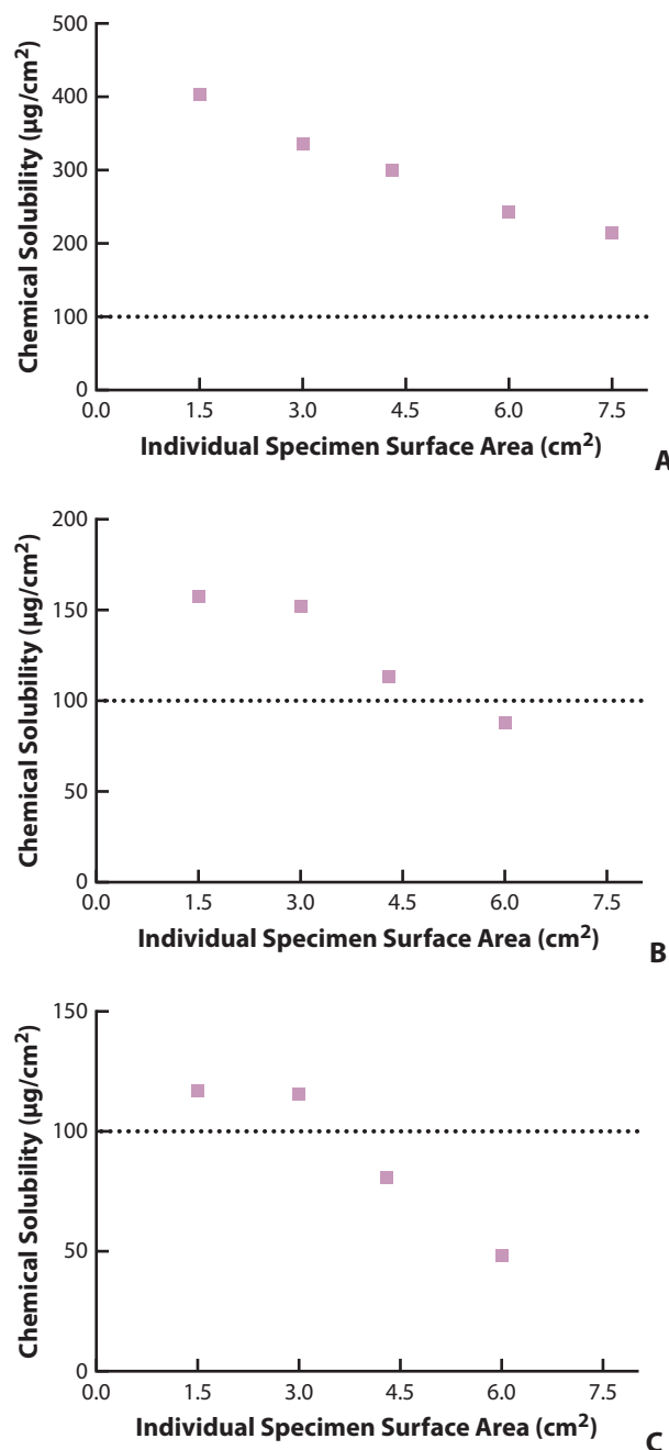
Figure 1. A, Relationship between chemical solubility rate and individual surface area of VITABLOCS Mark II. B, Relationship between chemical solubility rate and IPS e.max Press. C, Relationship between chemical solubility rate and IPS e.max ZirPress (cubes). Dotted line shows maximum acceptable chemical solubility (100 \mu\text{g}/\text{cm}^2 ) for enamel ceramics according to ISO 6872:2015 (bars represent standard deviation) ( n=1 ). Downward trend in chemical solubility rate with increasing individual specimen size observed for all materials. Statistical analysis showed significant difference among groups for each material tested ( P<.05 ).
