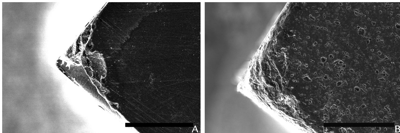
Figure 3. Scanning electron micrographs of VITABLOCS Mark II. A, Before solubility testing (surface, edge, and corner). B, After solubility testing (surface, edge, and corner). Scale bar equals 200 \mu\text{m} . Original magnification \times 500 .
