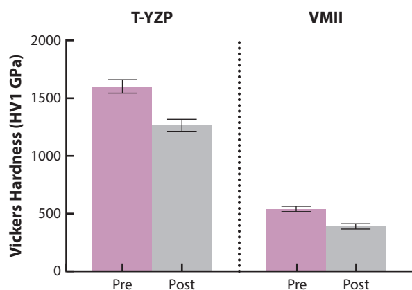
Figure 7. Difference of average hardness values of both Y-TZP and VITABLOCS Mark II specimens before and after chemical solubility tests (bars represent standard deviation) ( n=10 ).
