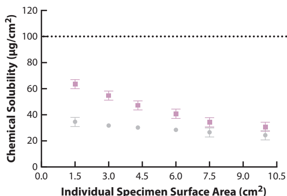
Figure 2. Comparison between average chemical solubility and individual surface area of Y-TZP cubes (black) and spheres (gray). Dotted line shows maximum acceptable chemical solubility (100 µg/cm²) for enamel ceramics according to ISO 6872:2015 (bars represent standard error) (n=3).
