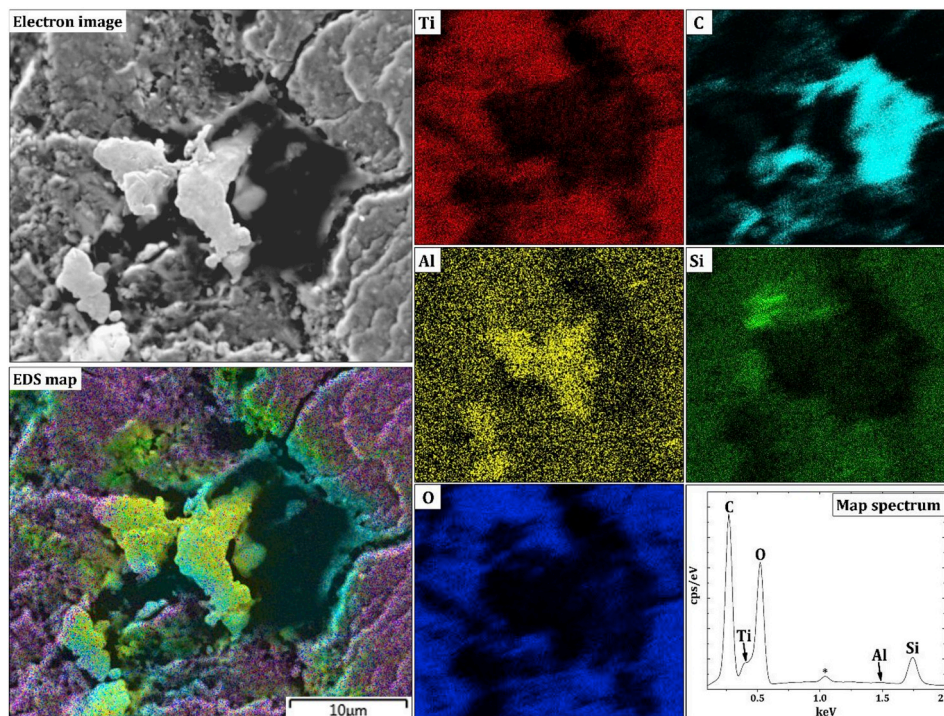
Fig. 21. SEM-EDS chemical map and spectrum taken from inside the wear track of \text{Ti}_3\text{SiC}_2 - \text{TiSi}_2 - \text{TiC}/\text{Al}_2\text{O}_3 tribo-pair for the test condition at 50 rpm.
