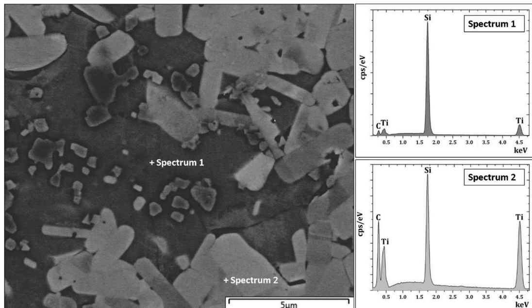
Fig. 7. EDS point spectrums showing the Ti-Si intermediate phase liquid region (spectrum 1) from which the growth of \text{Ti}_3\text{SiC}_2 (spectrum 2) occurred.
