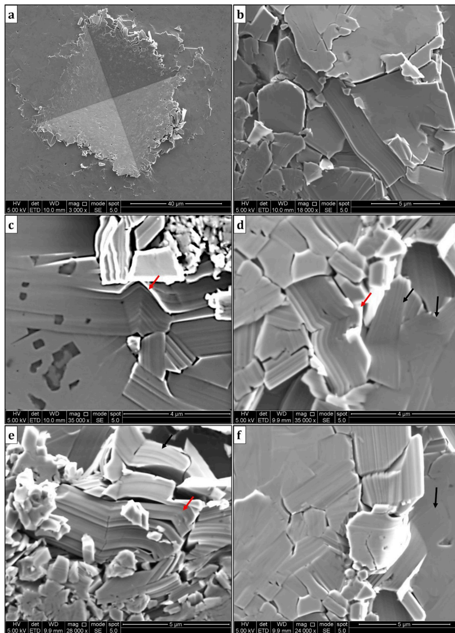
Fig. 10. SEM micrographs revealing the damage micromechanisms around the neighbourhood of the indentation prints created in the \text{Ti}_3\text{SiC}_2\text{-TiSi}_2\text{-TiC} composite. Note: In Fig.10(e) cavities are seen to have opened up between layers after extensive kink band formation.
