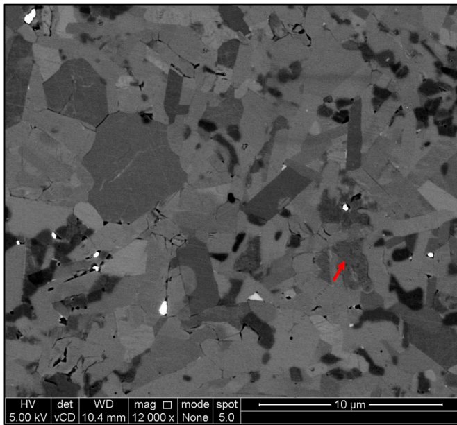
Fig. 5. A backscattered SEM micrograph of the unetched polished bulk sample. Note: white contrast are artefacts from colloidal silica used to reveal the microstructure without etching.
