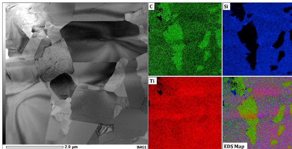
Fig. 14. STEM/EDS chemical mapping of the cross-sectional FIBed section from the worn surface.
