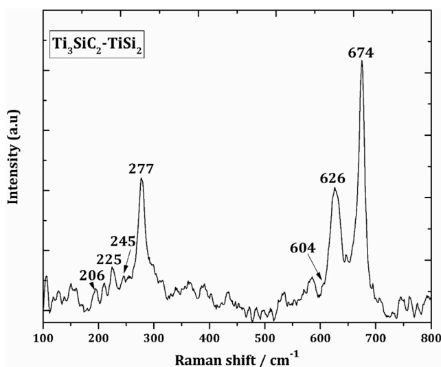
Fig. 19. Raman spectrum collected from the pristine surface of the \text{Ti}_3\text{SiC}_2 - \text{TiSi}_2 -TiC composite. Peaks at 206 \text{cm}^{-1} and 245 \text{cm}^{-1} correspond to the titanium disilicide vibrational modes.
