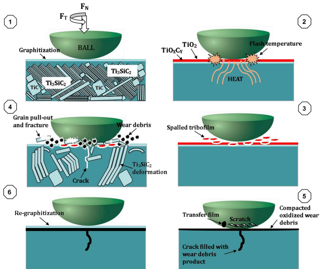
Fig. 24. Schematic presentation (1–6) showing the sequence of wear of the \text{Ti}_3\text{SiC}_2 - \text{TiSi}_2 - \text{TiC} MAX phase composite.
