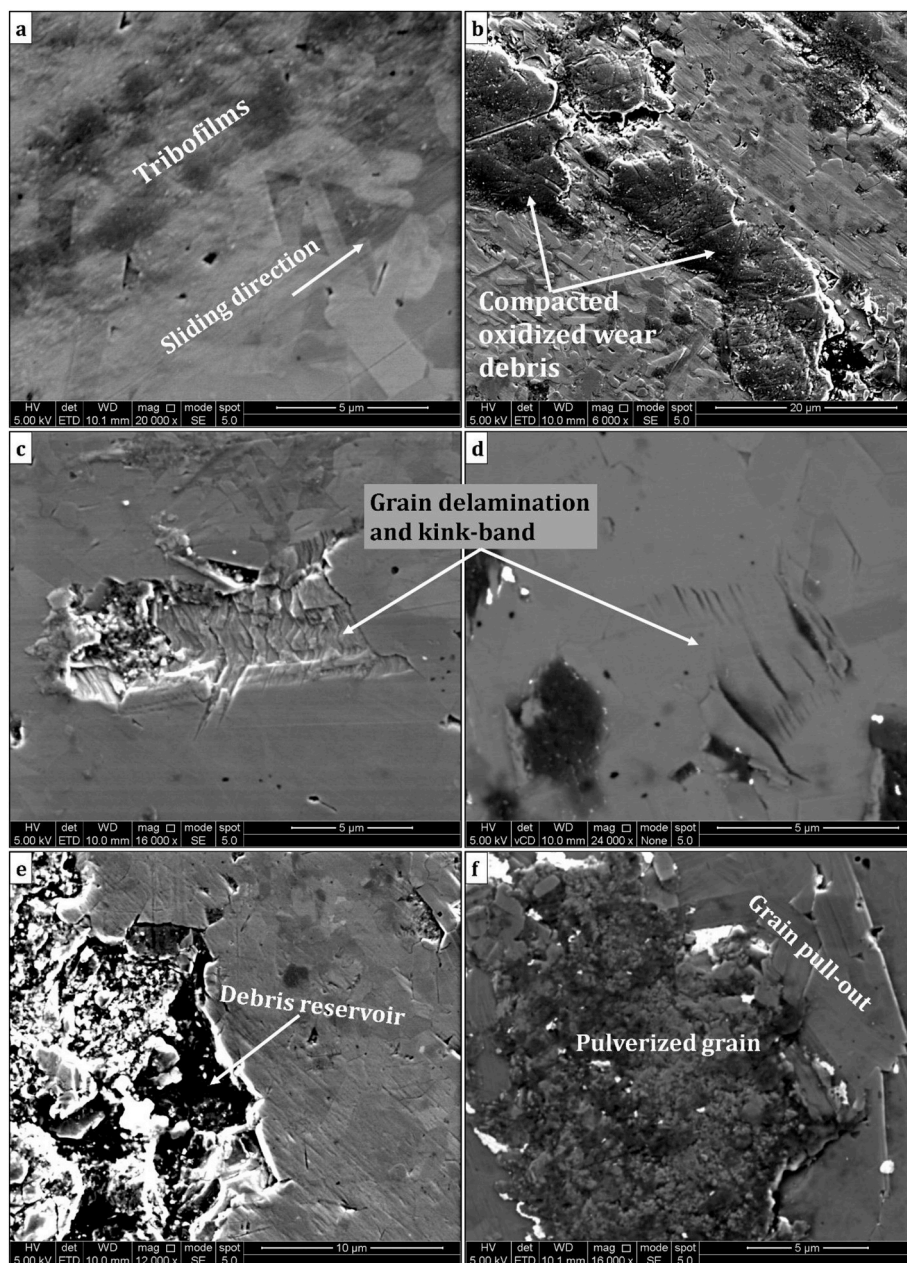
Fig. 13. Secondary electron (SE) SEM micrographs obtained from the worn surface of the disc.
