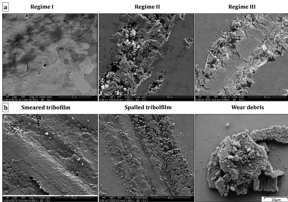
Fig. 22. (a) Evolution of surface microstructures corresponding to regimes I–III, and (b) details of surface microstructure leading to transition from regime I–II as observed in the friction plot for the test conducted at 50 rpm.
