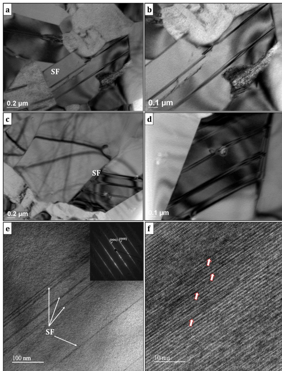
Fig. 15. Bright-field (BF) TEM micrographs showing extensive stacking fault (SF) propagation across the \text{Ti}_3\text{SiC}_2 grains: (b) is a higher magnification of (a), (d) is a higher magnification of (c), (e) bright-field (STEM) revealing stacking faults across a \text{Ti}_3\text{SiC}_2 grain with inset showing corresponding SAED pattern and (f) HRTEM image taken from the \text{Ti}_3\text{SiC}_2 grain.
