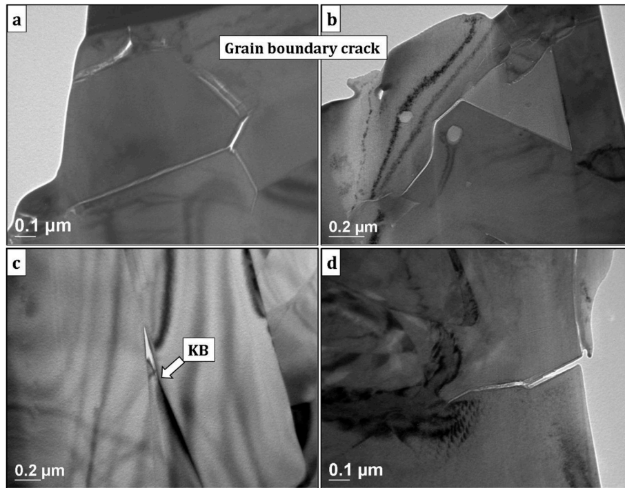
Fig. 16. Bright-field (BF) TEM images showing: (a–b) grain boundary cracks, (c) kink band (KB) containing crack along the kink boundary and (d) crack propagating across the \text{Ti}_3\text{SiC}_2 grain.
