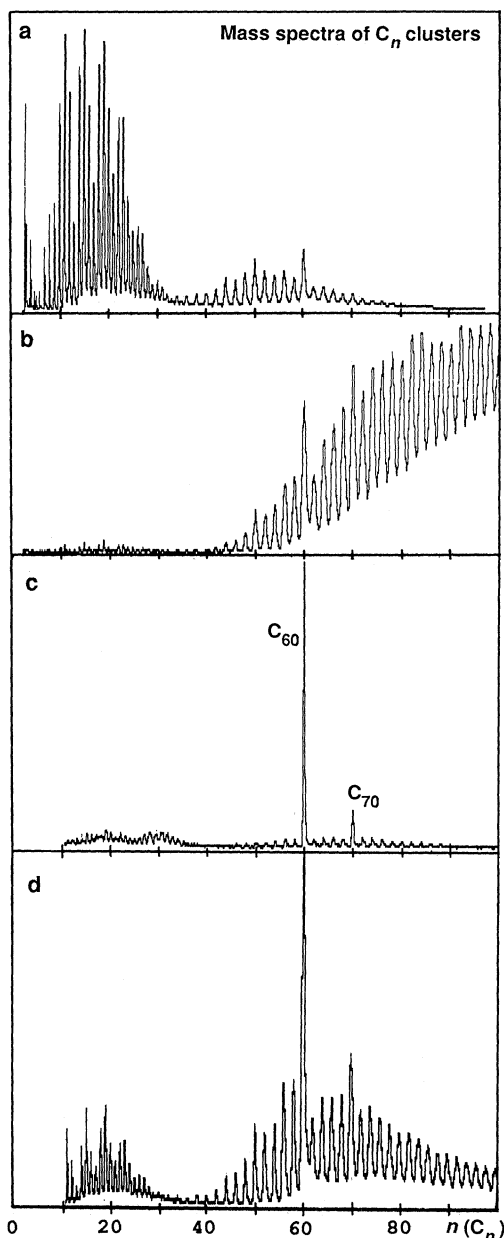
Fig. 2. Mass spectra under various conditions. (a) Moderate clustering: both polyne chain precursors ( n < 36 ) and fullerenes ( n > 20 ) observed. (b) Significant clustering: only even clusters (all fullerenes?) detected. (c) Extensive clustering: C_{60} and C_{70} remain and appear to be dominant because the very large clusters are well above the detection range. (d) Clustering similar to (c) but at about 100 times the ionizing laser flux: extensive fragmentation of large clusters (particles) into fullerenes and chain precursors occurs.
