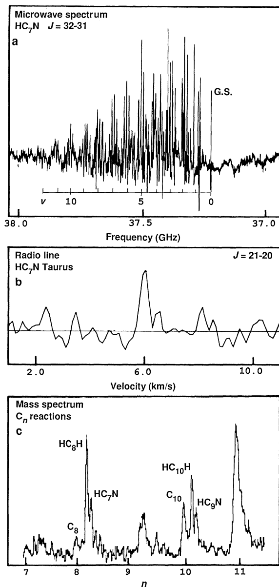
Fig. 1. Data on H-C≡C-C≡C-C≡C-C≡N. (a) A microwave rotational transition; J , rotational quantum number; \nu , lowest binding vibrational quantum number. The “vibrationless” ground-state line is at the far right, G.S. ( \nu = 0 ). Most of the molecules are, however, flexing violently as indicated by the multitude of bending vibrational satellites (all the other lines with \nu > 0 ). This is the quantum picture of the rotation/flexing process. (b) A rotational line detected by radio astronomy from a molecular cloud with a Doppler velocity of 6 km/s in the constellation of Taurus. (c) The mass spectrum of the C/H/N reaction. The bare C 8 and C 10 peaks (at 8 \times 12 and 10 \times 12 amu positions, respectively) develop satellites at +2 amu for HC 8 H and HC 10 H and at +3 amu for HC 7 N and HC 9 N, respectively.
