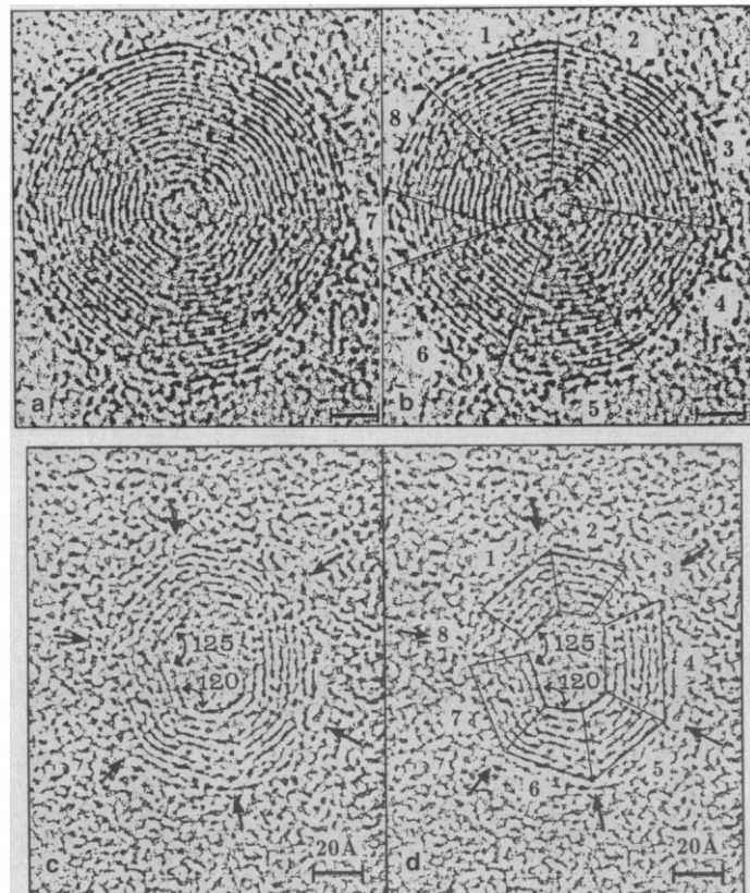
Fig. 8. Particles photographed by Sumio Iijima (44) which show clear evidence of polyhedral concentric shell structure consistent with the icospiral graphite particle model. At the right the contours are delineated.
