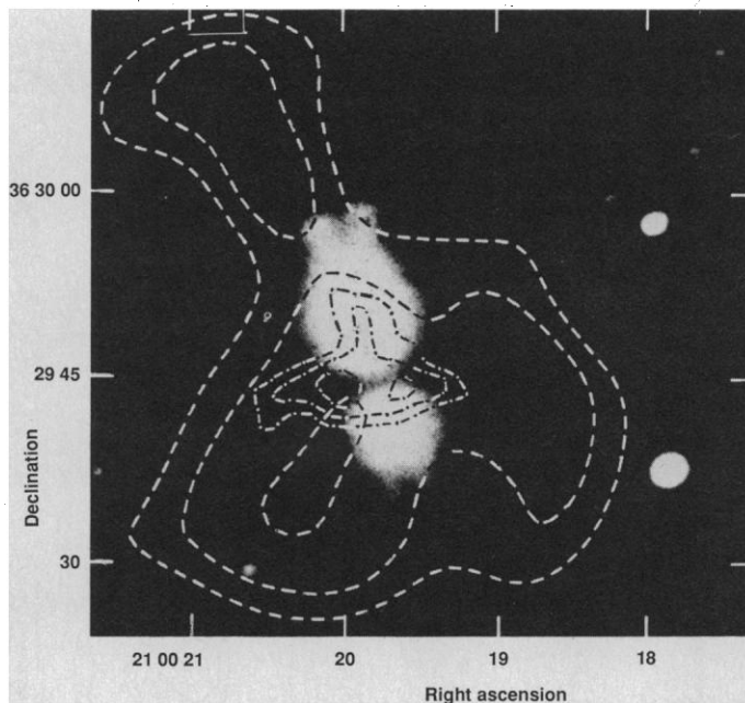
Fig. 10. Map of HC_7N (---) and NH_3 (-·-·-) from Rieu et al. (54) superimposed on a photograph of the Egg Nebula scattering (55). The dust emanates in two lobes from a central star. These data suggest that HC_7N results from fragmentation of carbonaceous dust by starlight; compare with Fig. 2d. Laboratory data (Fig. 2) indicate that even carbon clusters, in particular C_{60} (most likely ionized as C_{60}^+ ), must be present along with chains.
